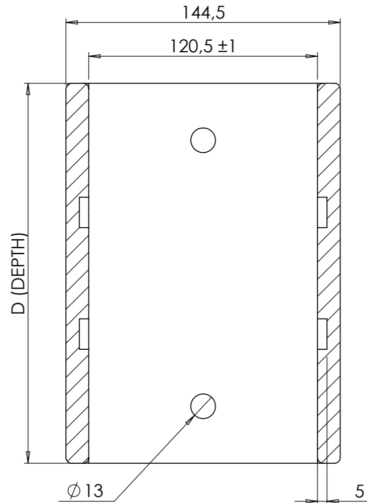
SECTION B-B
