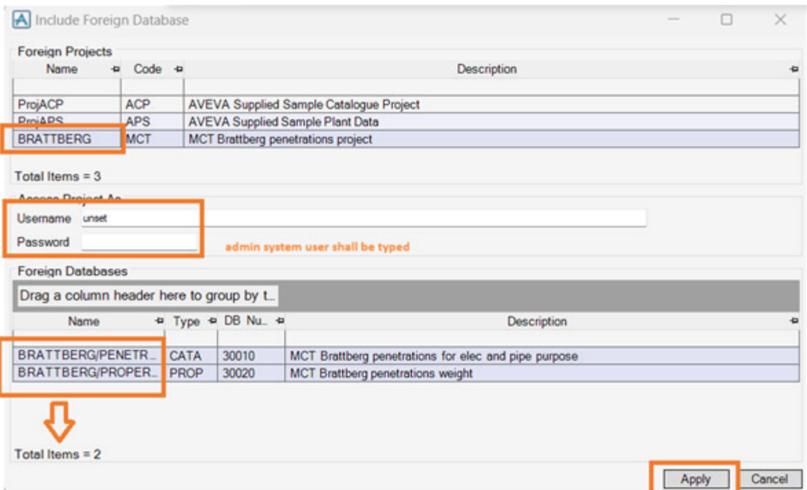
Figure 2. AVEVA Administration with “Include Foreign Database”.
